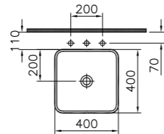
COUNTERTOP
